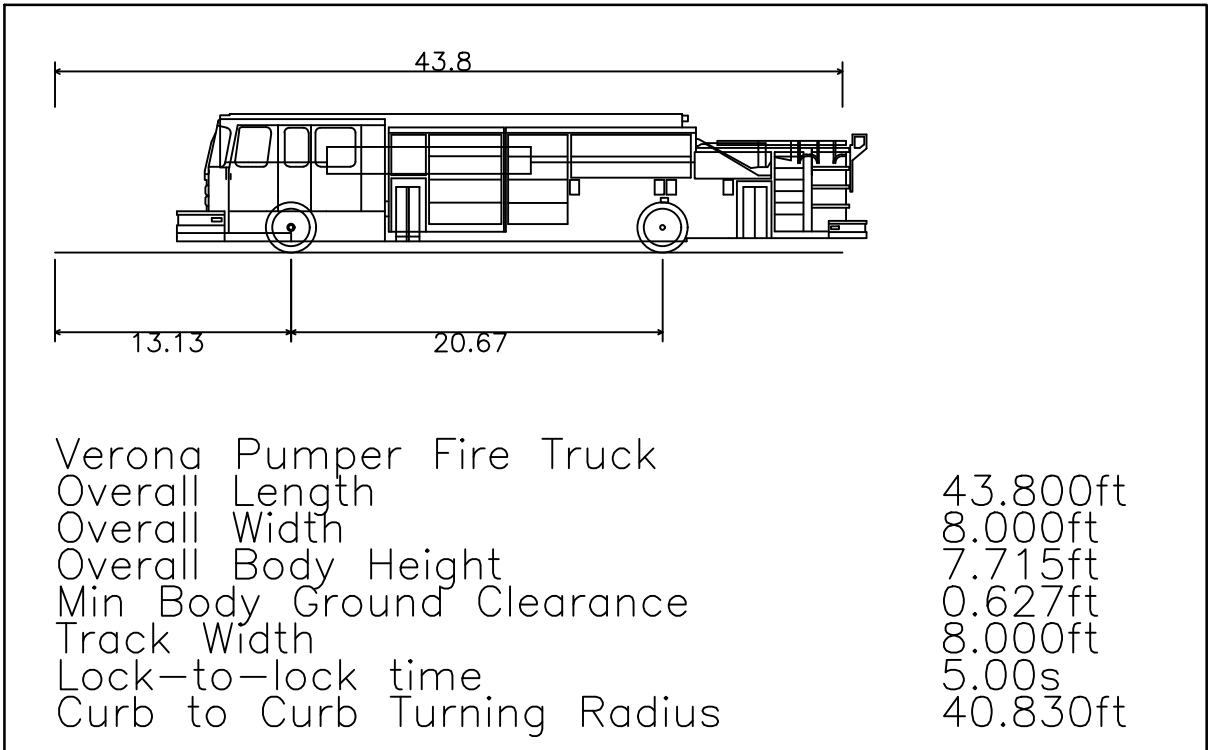
VERONA PUMPER FIRE TRUCK DETAIL NOT TO SCALE
