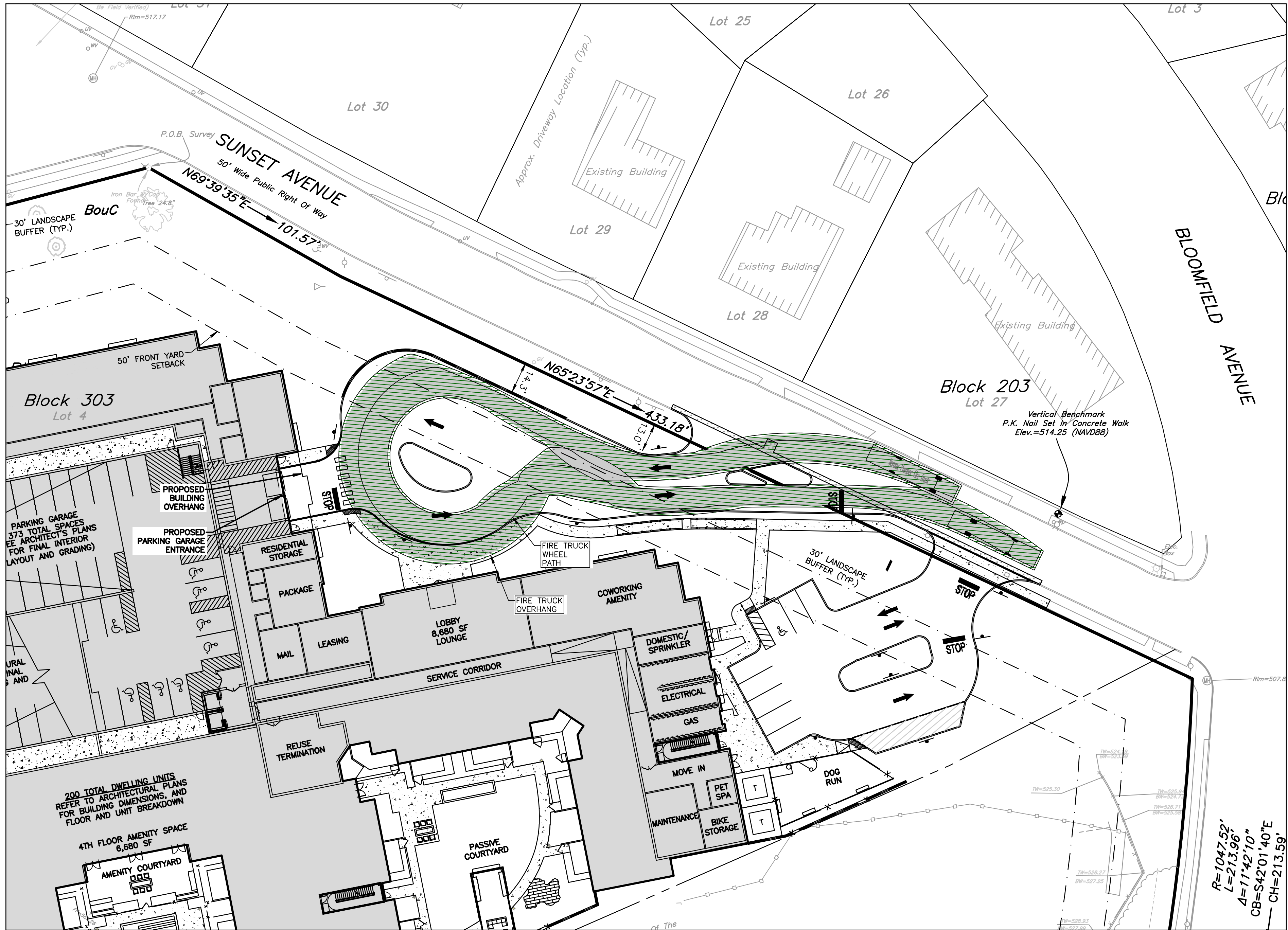
VERONA FIRE TRUCK TURNING PLAN — MODIFIED CIRCLE LAYOUT SCALE 1" = 30'
